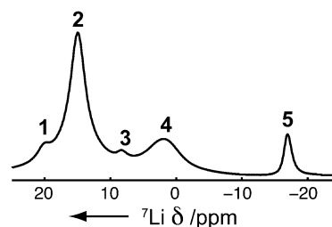
Figure 4. ^7\text{Li} NMR spectrum of \text{Li}_{12}\text{Si}_7 at 233 K. See text for details.
